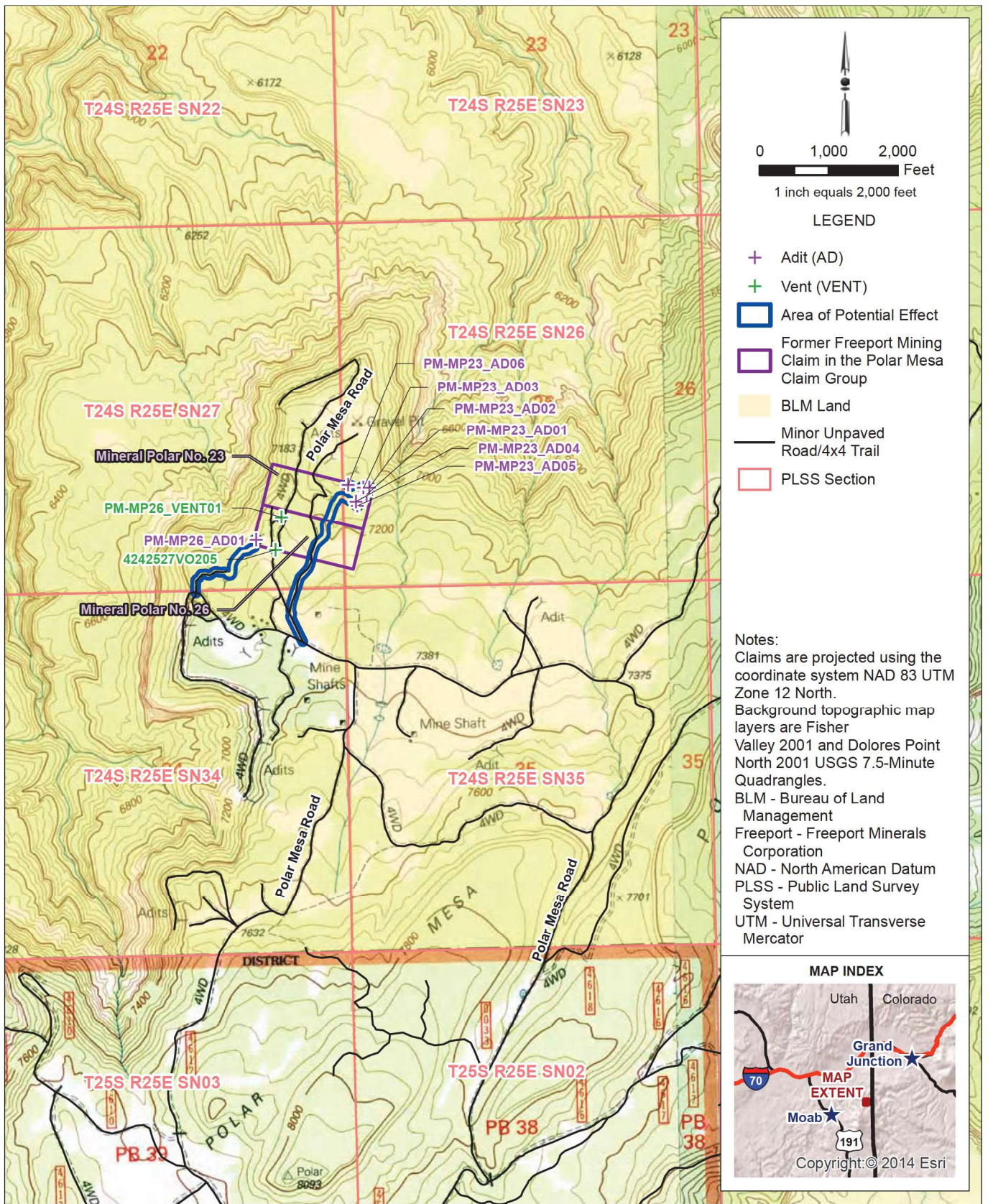
FIGURE 2 GATEWAY MINING DISTRICT PROPOSED CLOSURES SITE MAP FREEPORT MINERALS CORPORATION PROPOSED MINE FEATURE CLOSURES – YELLOW CAT AND GATEWAY MINING DISTRICTS, UTAH
