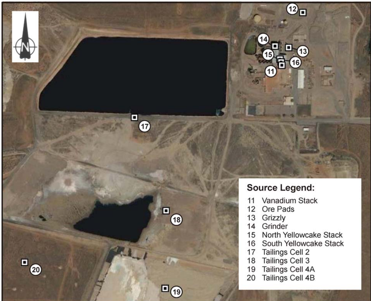
FIGURE 4.1 SOURCE LOCATIONS
